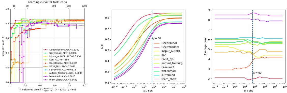
(a) Learning curves for the task Carla (b) Impact of t_0 on the ALC scores for task Carla . (c) Average rank among AutoDL final phase participants, using different t_0 . The legend is hidden and is the same as that of Figure 10b.
