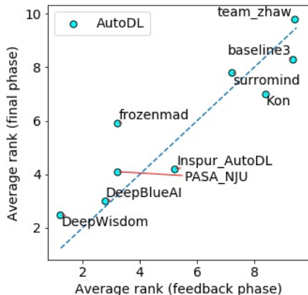
Fig. 9: Task over-modeling: We compare performance in the feedback and the final phase, in an effort to detect possible habituation to the feedback datasets due to multiple submissions. The average rank of the top-8 teams is shown. The figure suggests no strong over-modeling (over-fitting at the meta-learning level): A team having a significantly better rank in the feedback phase than in the final phase would be over-modeling (far above the diagonal). The Pearson correlation is \rho_{X,Y} = 0.91 and p -value p = 5.8 \times 10^{-4} .
