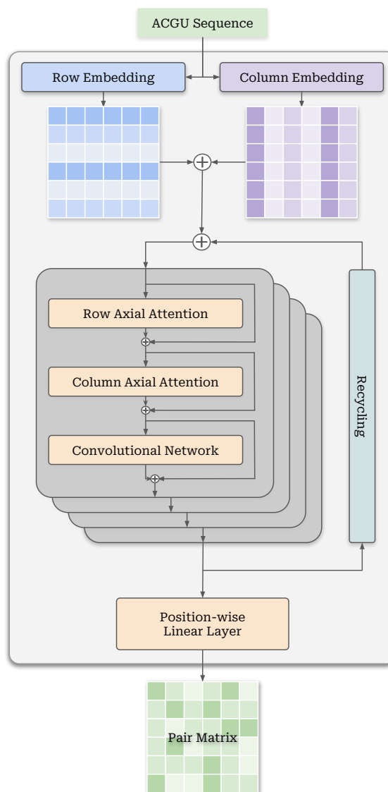
Figure 1. An overview of the RNAformer architecture.
