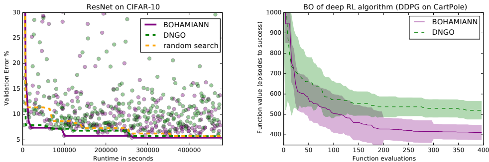
Figure 2: (Left) DNGO vs. BOHAMIANN for optimizing the 8 hyperparameters of a deep residual network on CIFAR-10; we plotted each function evaluation performed over time, as well as the current best; parallel random search is included as an additional baseline. (Right) DNGO vs. BOHAMIANN for optimizing the 12 hyperparameters of an RL agent.
